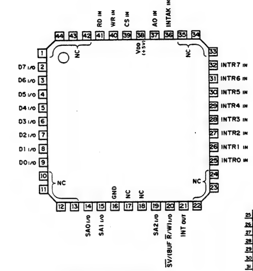
UPD71059G (NEC) FLAT PACKAGE C-MOS INTERRUPT CONTROL UNIT — TOP VIEW —
